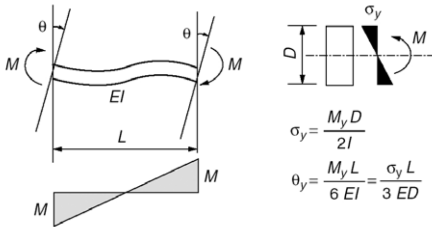
Fig. 4 Deformation angle at beam ends of a rigid frame.
