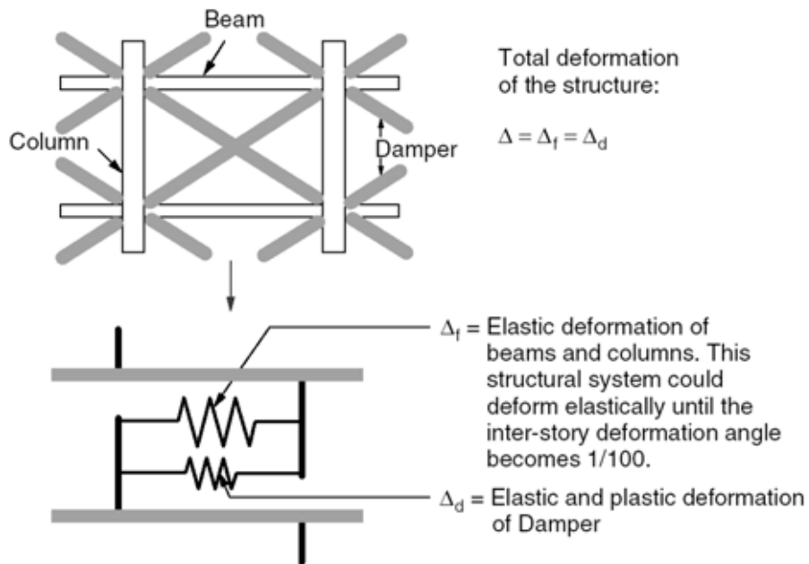
Fig. 6 Structure with dampers.
