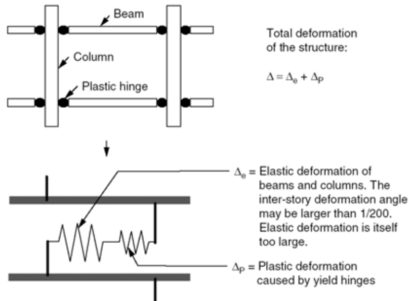
Fig. 2 Strong column weak beam model.
