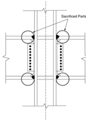
Fig. 1 Typical beam-column connection in the United States before Northridge earthquake.
