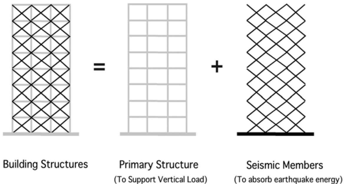
Fig. 5 Concept of damage-controlled structures.
